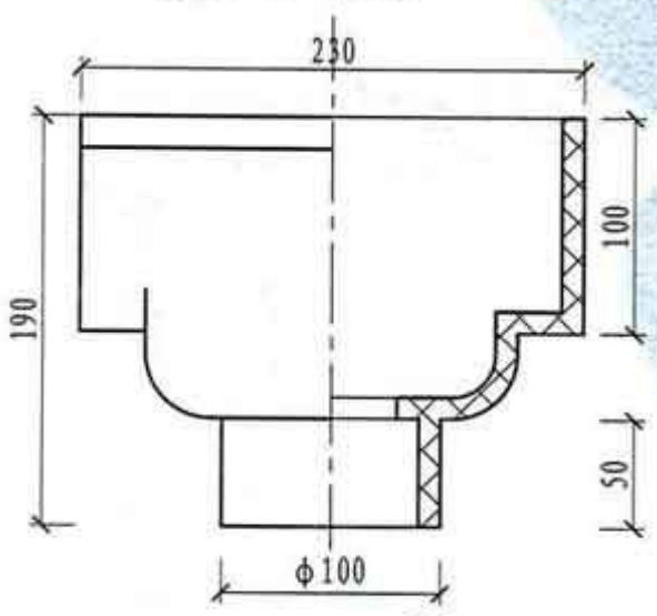
③ UPVC方雨水斗
