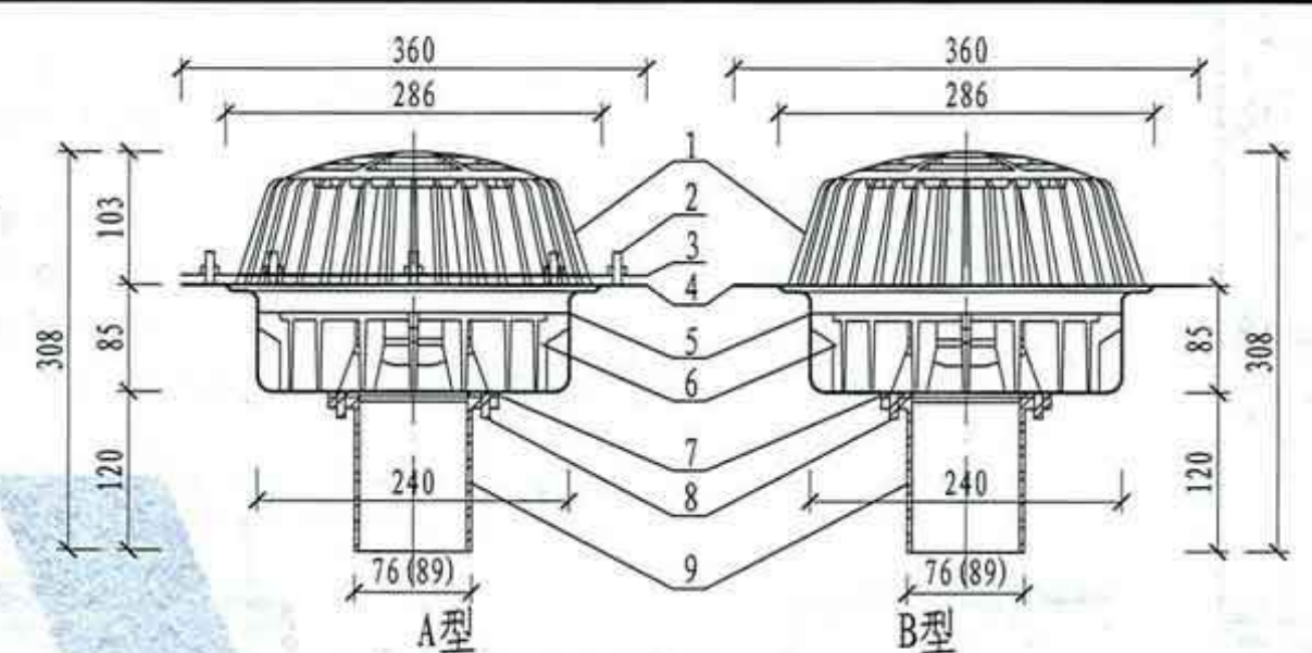
② YG75 (80)型虹吸式雨水斗
