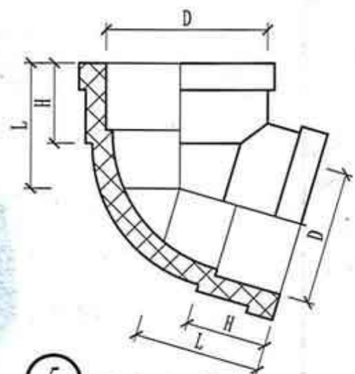
UPVC45°弯头透视
